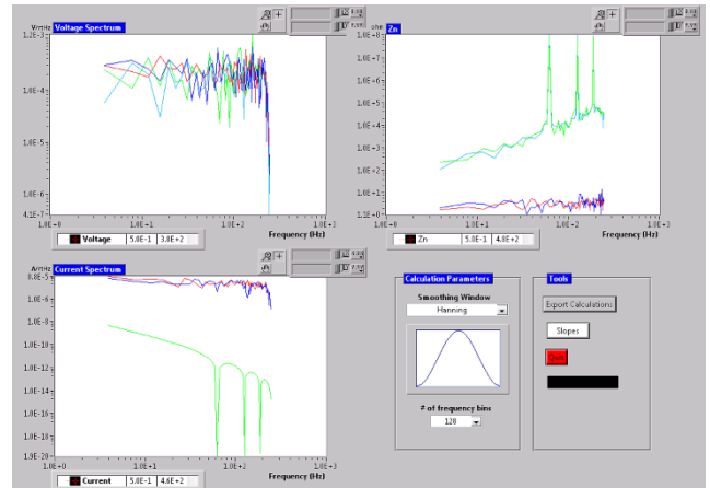
Figure 4. Fourier analysis of four different experimental conditions: Blue, shielded cables and no motor; red, shielded cables with motor; light blue, unshielded cables and no motor; green, unshielded cables with motor. Top left is the voltage PSD, bottom left is current PSD, and top right is impedance PSD.
